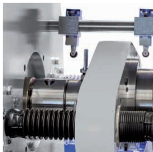
Simple adjustment of the moveable cone system allows a fast and trouble free start up and shut down of the press and for pressure regulation.
